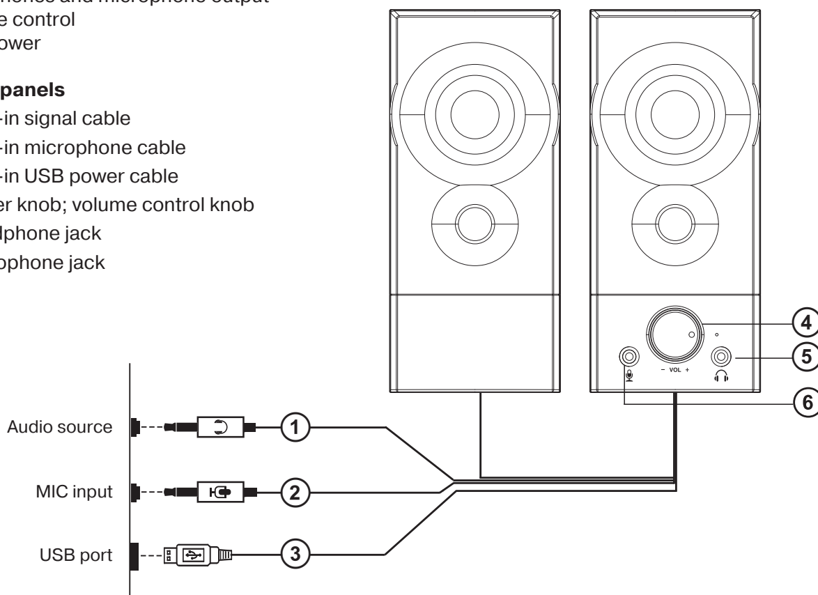
Fig. 1. Connection diagram
